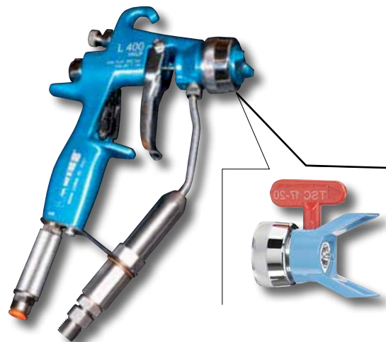
Mist-less manual gun L400 complete with Super Fast Clean or Top Spraying Clean nozzle with long filter
